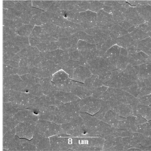
Fig. 4: Microcracks on the surface of the ablation bottom.
