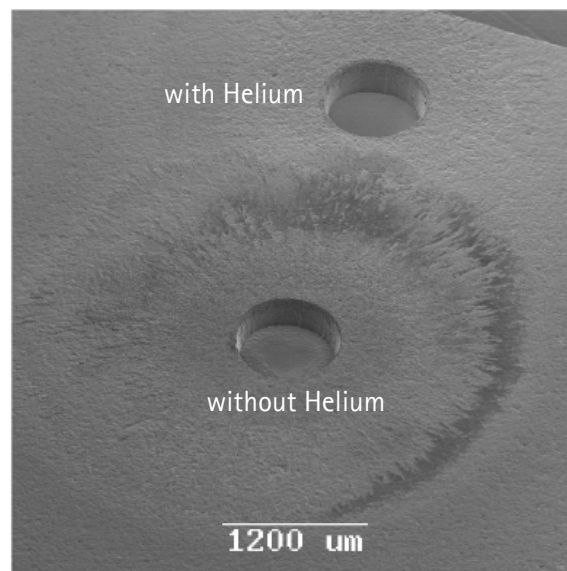
Fig. 3: Ablations of sapphire with (above) and without (below) Helium as inert gas.
