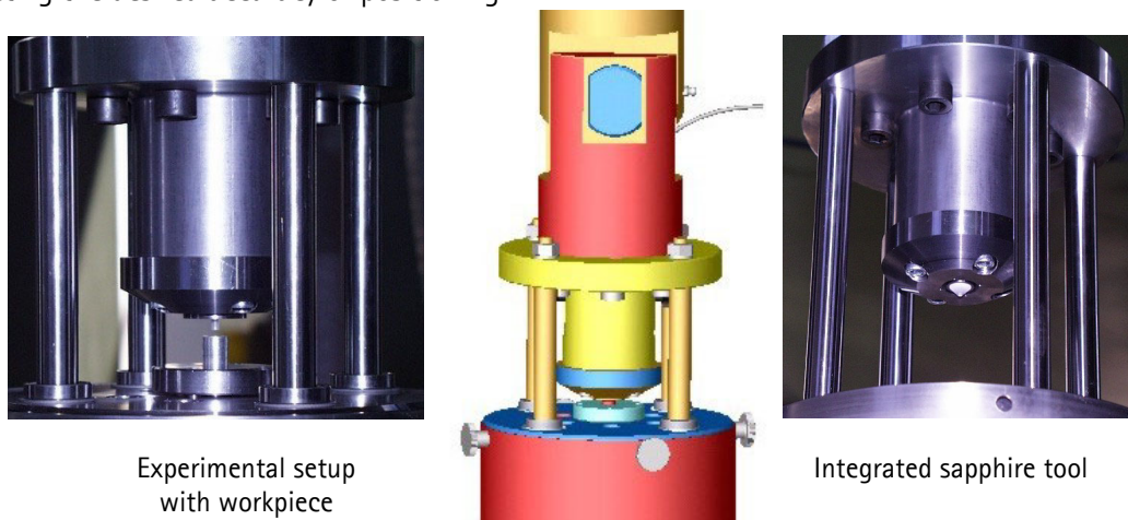
Fig. 5: Prototype of a setup for laser-assisted microforming
