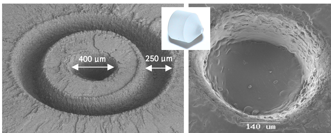
Fig. 7: Sapphire tool for embossing experiments
