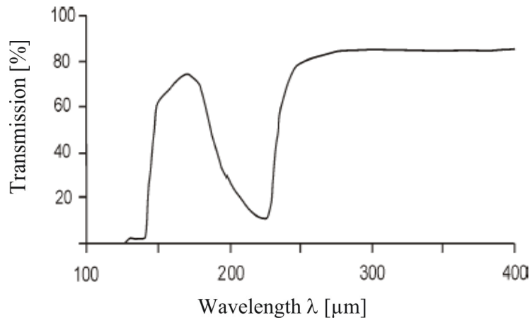
Fig. 2: Transmission curve of sapphire
