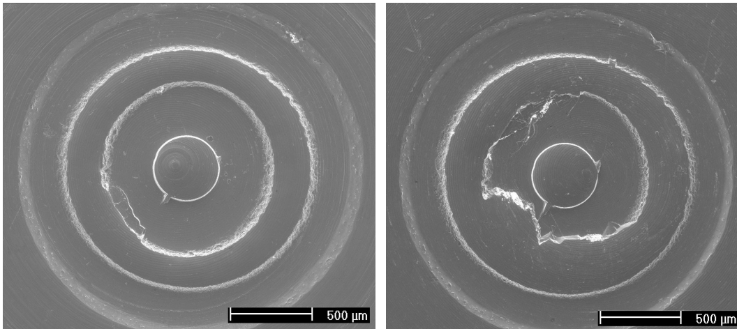
Fig. 9: Results of the embossing experiments: imprints in stainless steel 1.4301
