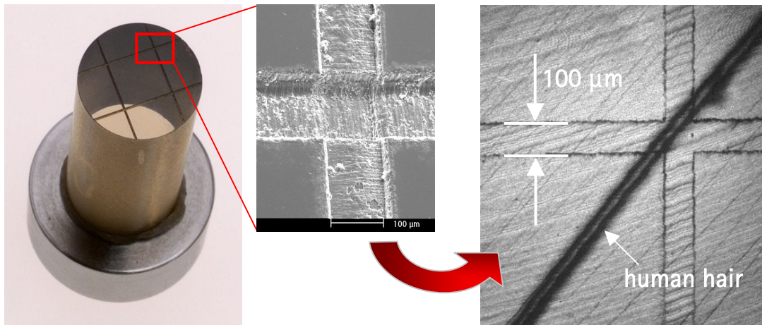
Fig. 6: Prototype of a sapphire tool for embossing and imprint in aluminium
