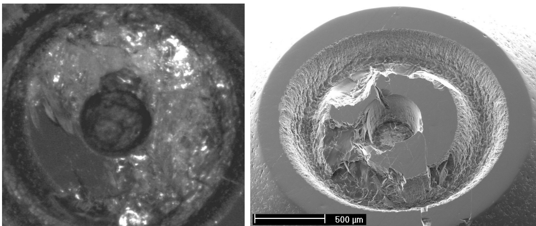
Fig. 10: Sapphire tool fractured during the embossing experiments
