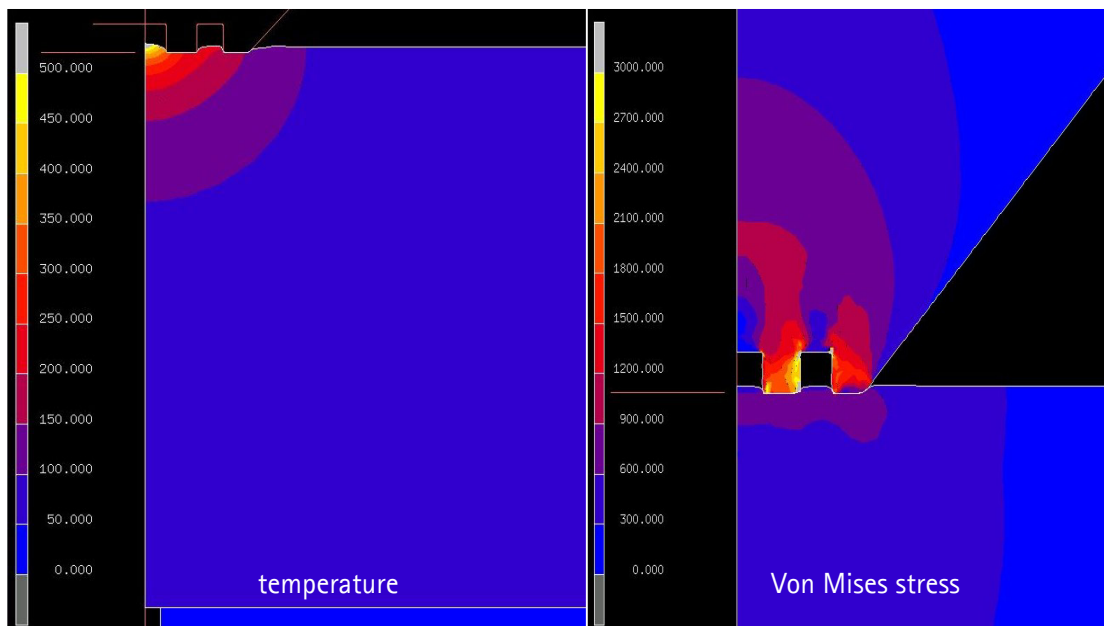
Fig. 8: Results of FE simulations of the embossing experiments
