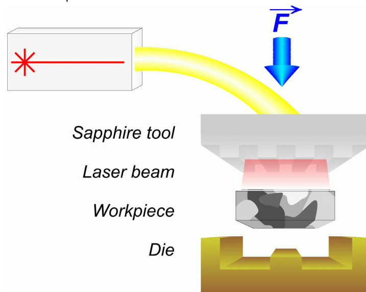
Fig. 1: Principle of laser-assisted microforming
